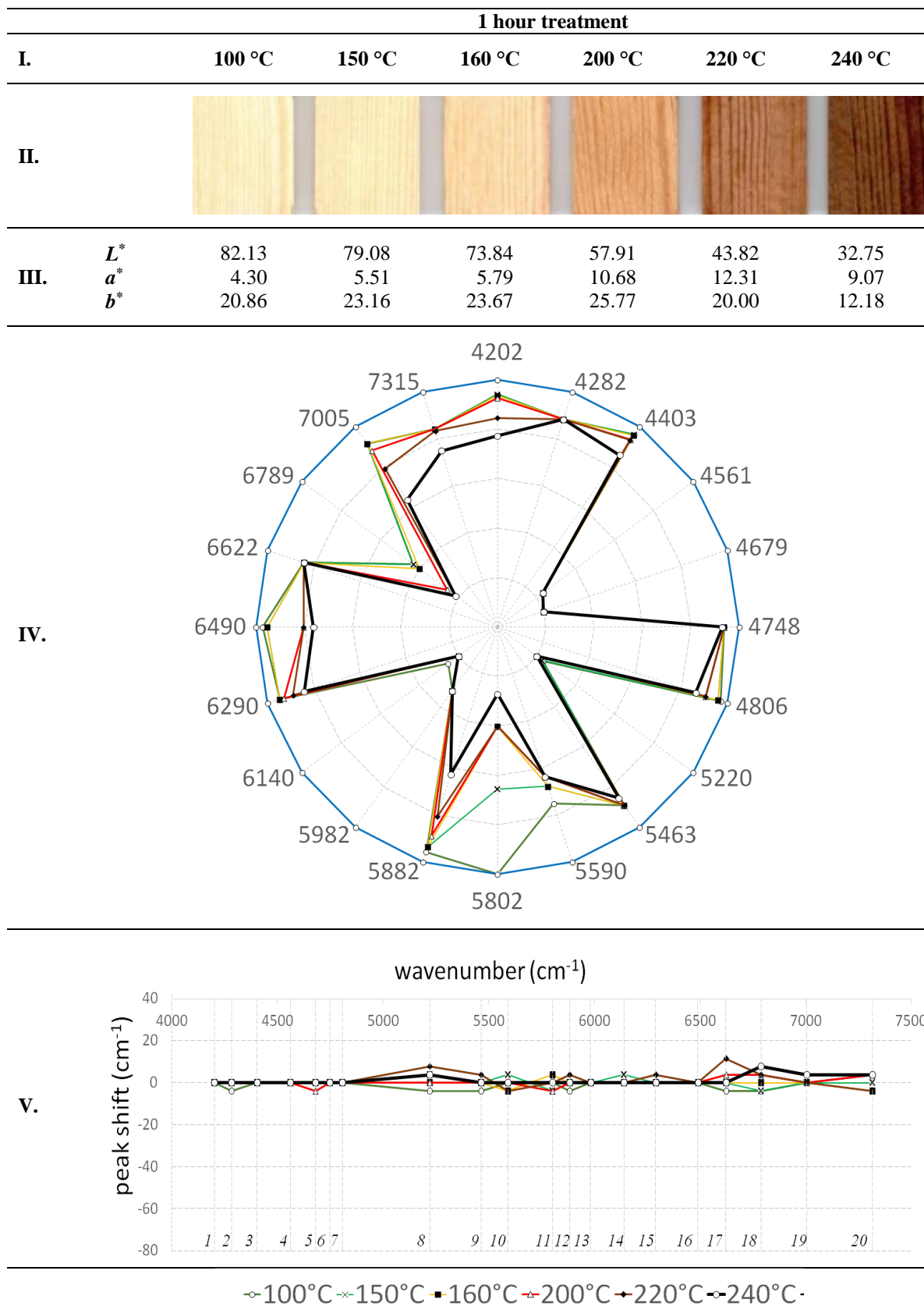
Fig. 3 Summary results for 1 hour heat treatment of pine sapwood.
