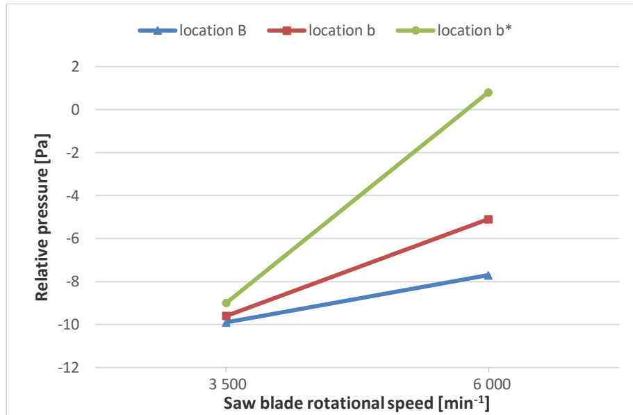
Fig. 10 Relative pressure [Pa] as a function of saw blade rotational speed at different location for wide and narrow cover; saw blade No. 1 ( \varnothing 300 mm), fan motor frequency 50 Hz.
