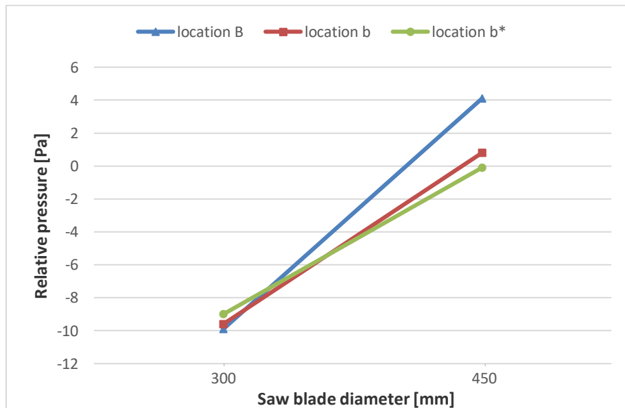
Fig. 11 Relative pressure [Pa] as a function of saw blade diameter at different location for wide and narrow cover; saw blade rotational speed 3500 \text{ min}^{-1} , fan motor frequency 50 Hz.
