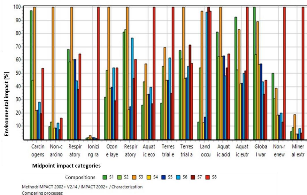
Fig. 11 Characterization of S1- S8 structure assemblies, SimaPro, IMPACT2002+.
