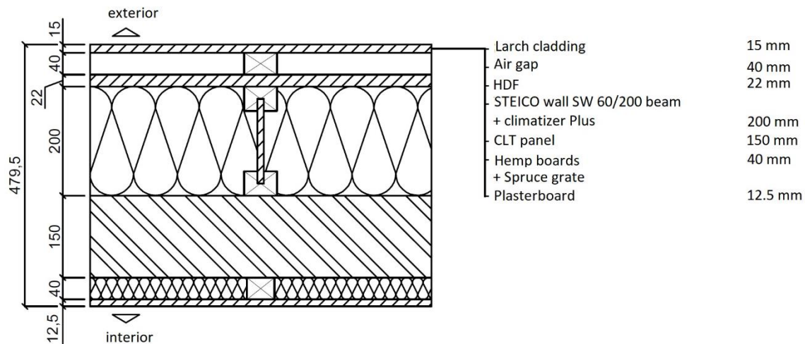
Fig 8. Cross-section and materials in the assembly of the S8 structure.
