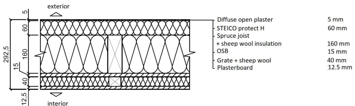
Fig 7. Cross-section and materials in the assembly of the S7 structure.
