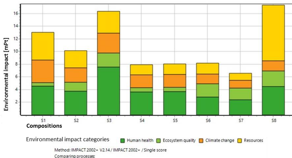
Fig. 16 LCIA of S1- S8 structure assemblies, endpoints (mPt), SimaPro, IMPACT2002+.
