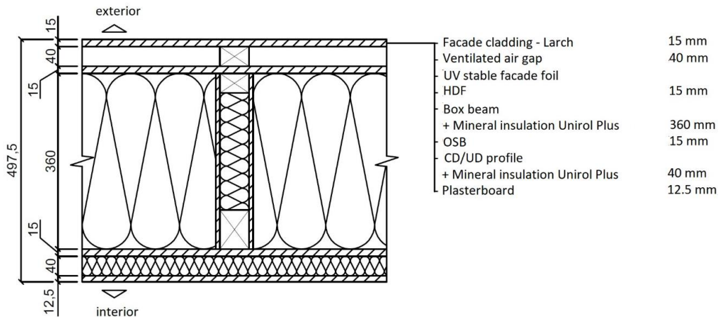
Fig 3. Cross-section and materials in the assembly of the S3 structure.
