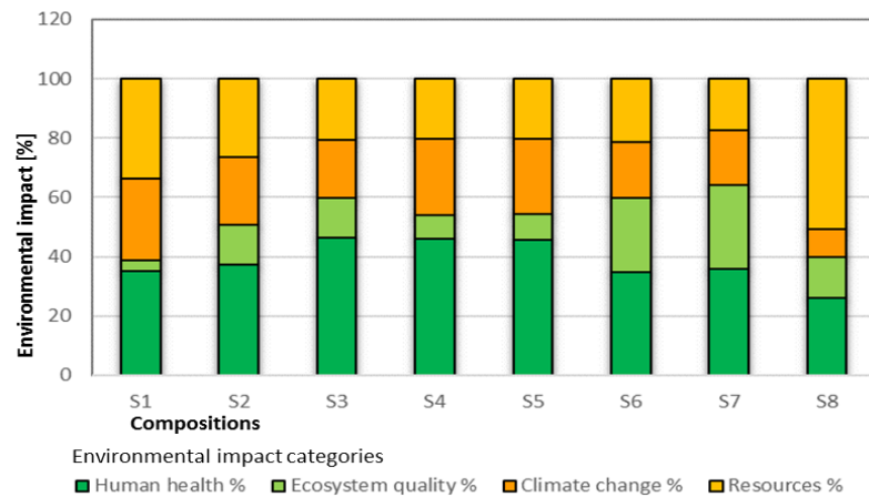
Fig. 15 LCIA of the S1- S8 structure assemblies, endpoints (%), SimaPro, IMPACT2002+.
