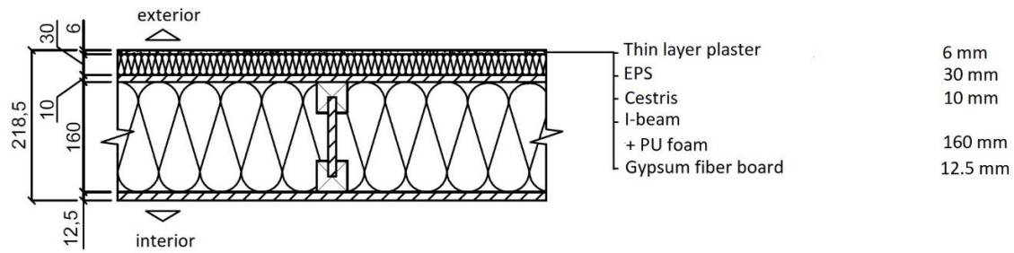
Fig 1. Cross-section and materials in the assembly of the S1 structure.
