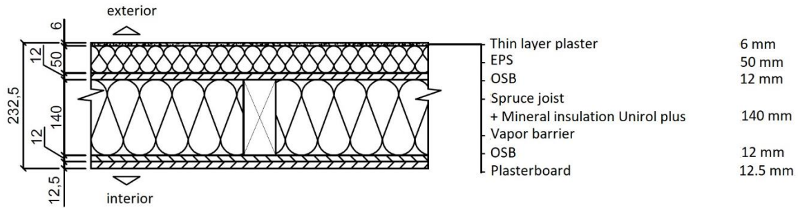
Fig 2. Cross-section and materials in the assembly of the S2 structure.
