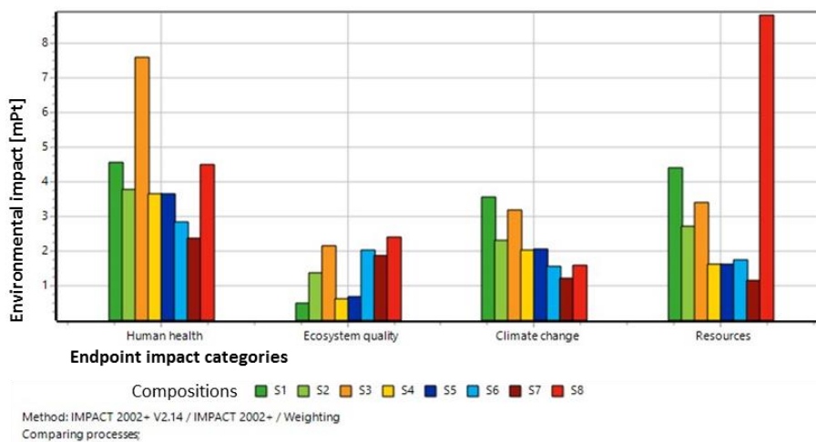
Fig. 14 Weighting S1- S8 structure assemblies, SimaPro, IMPACT2002+.
