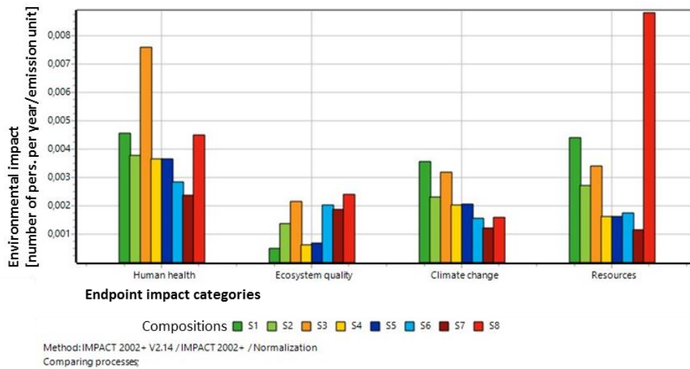
Fig. 13 Normalization of S1- S8 structure assemblies, SimaPro, IMPACT2002+.
