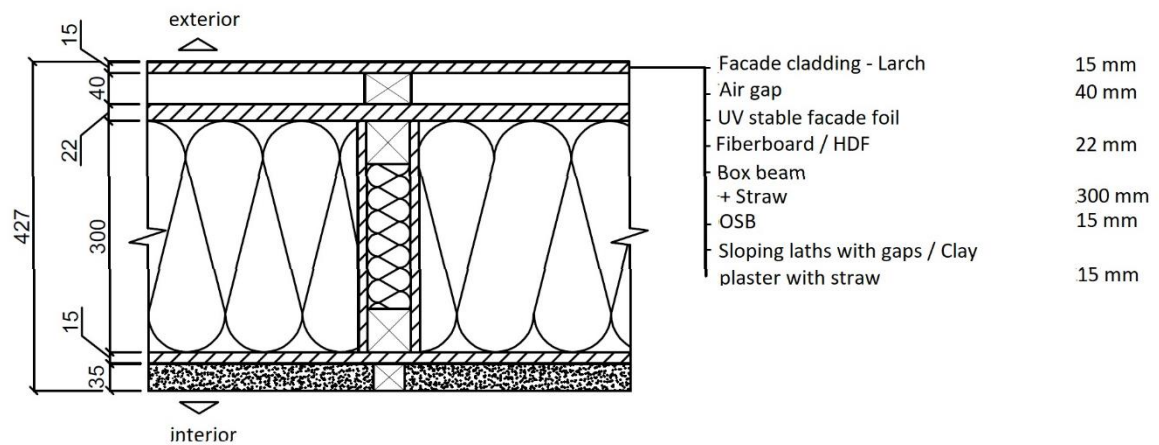
Fig 6. Cross-section and materials in the assembly of the S6 structure.
