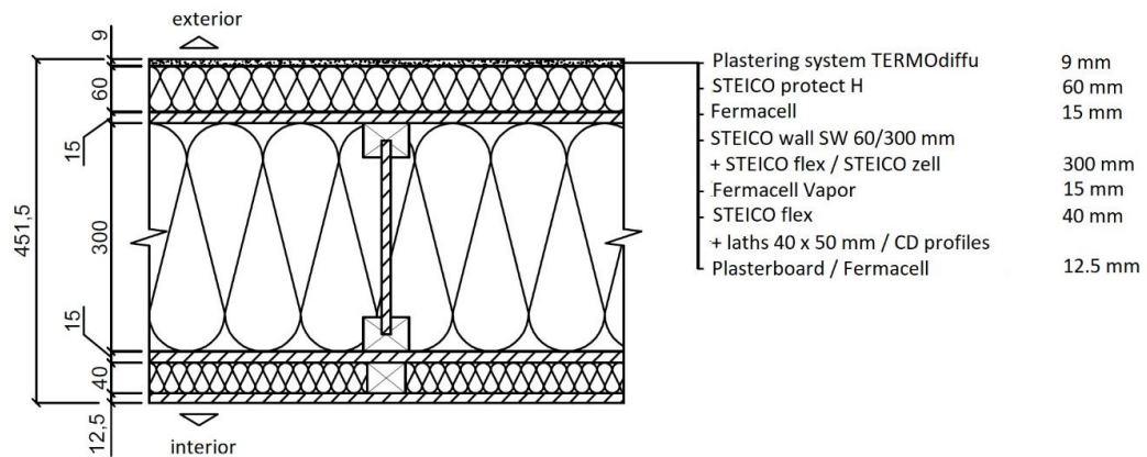
Fig 5. Cross-section and materials in the assembly of the S5 structure.
