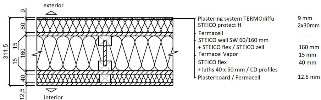
Fig 4. Cross-section and materials in the assembly of the S4 structure.
