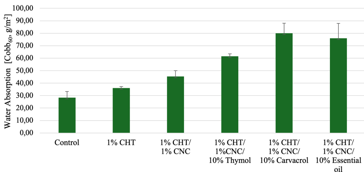
Fig. 2: Cobb 60 values (g/m 2 ) of uncoated and treated paperboard samples
