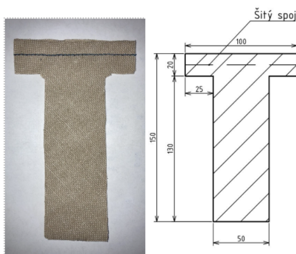
Fig. 2 Shape and dimensions of the test specimen for determining the strength of the sewn seam (authors' archive, STN EN ISO 13935-1:2001)
