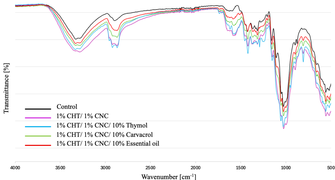
Fig. 4: The ATR-FTIR spectra of samples
