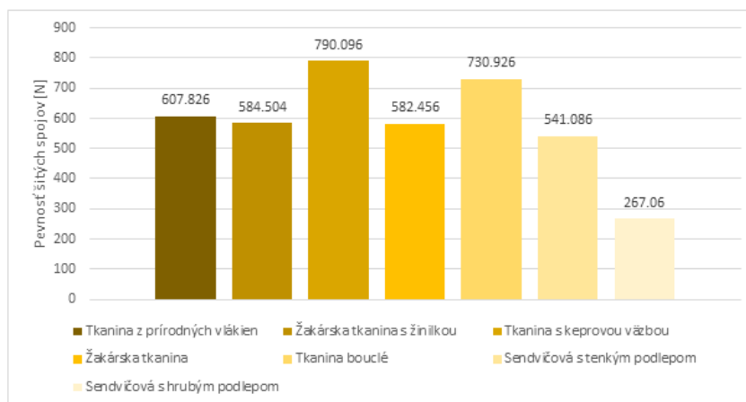
Fig. 7 Strength of sewn seams in diagonal joining of textiles
