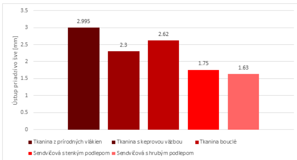
Fig. 8 Yarn slippage in the seam in diagonal joining
