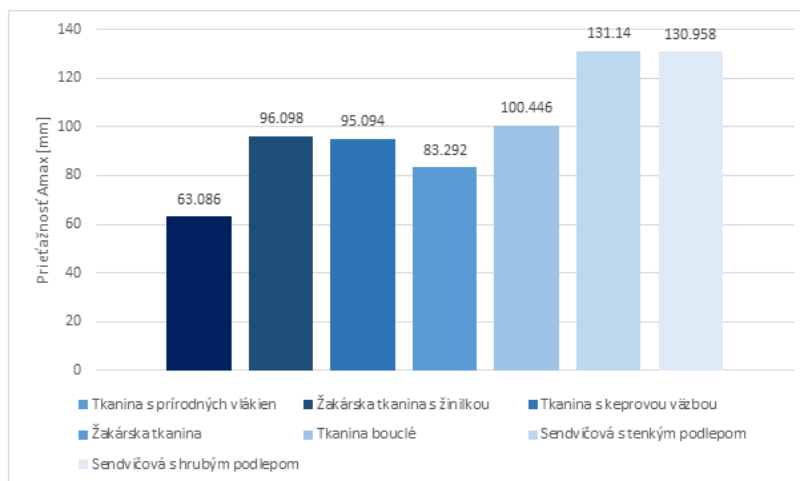
Fig. 6 Elongation of fabrics in the diagonal direction
