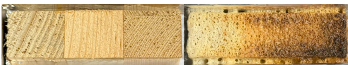
Obr. 3 Porovnanie neošetrenej a ošetrenej vzorky pri teplote 150 °C na konci merania Fig. 3 Comparison of non-treated and treated sample at 150 °C at the end of measurement
