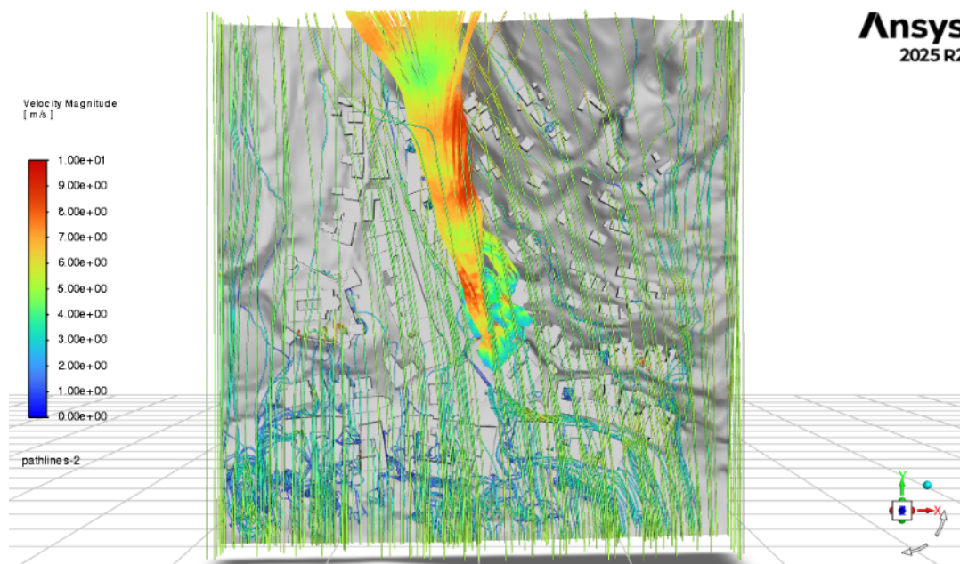
Obr. 7 Zobrazenie smeru vetra a dymu pomocou Pathlines Fig. 7 Wind Direction and Smoke Dissipation Displayed by Pathlines
