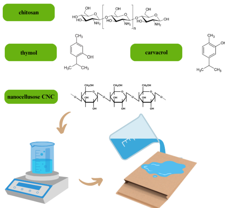
Fig. 1: Preparation scheme of coated paperboard
