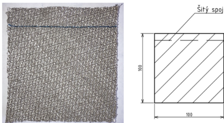
Fig. 3 Shape and dimensions of the test specimen for determining yarn slippage (authors' archive)
