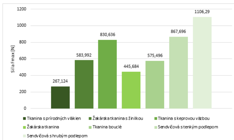
Fig. 5 Tensile strength of fabrics in the diagonal direction
