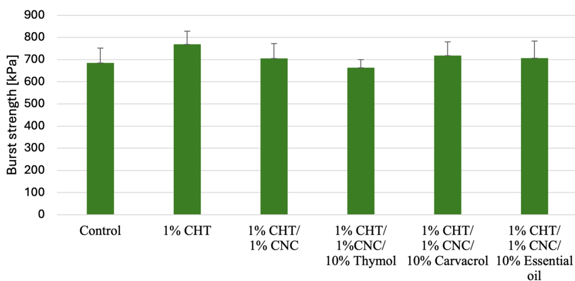
Fig. 3: Burst strength (kPa) of uncoated and treated paperboard samples
